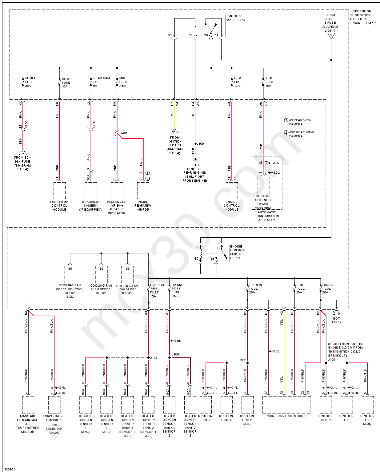
Fig. 52: Power Distribution Circuit (4 of 4)
