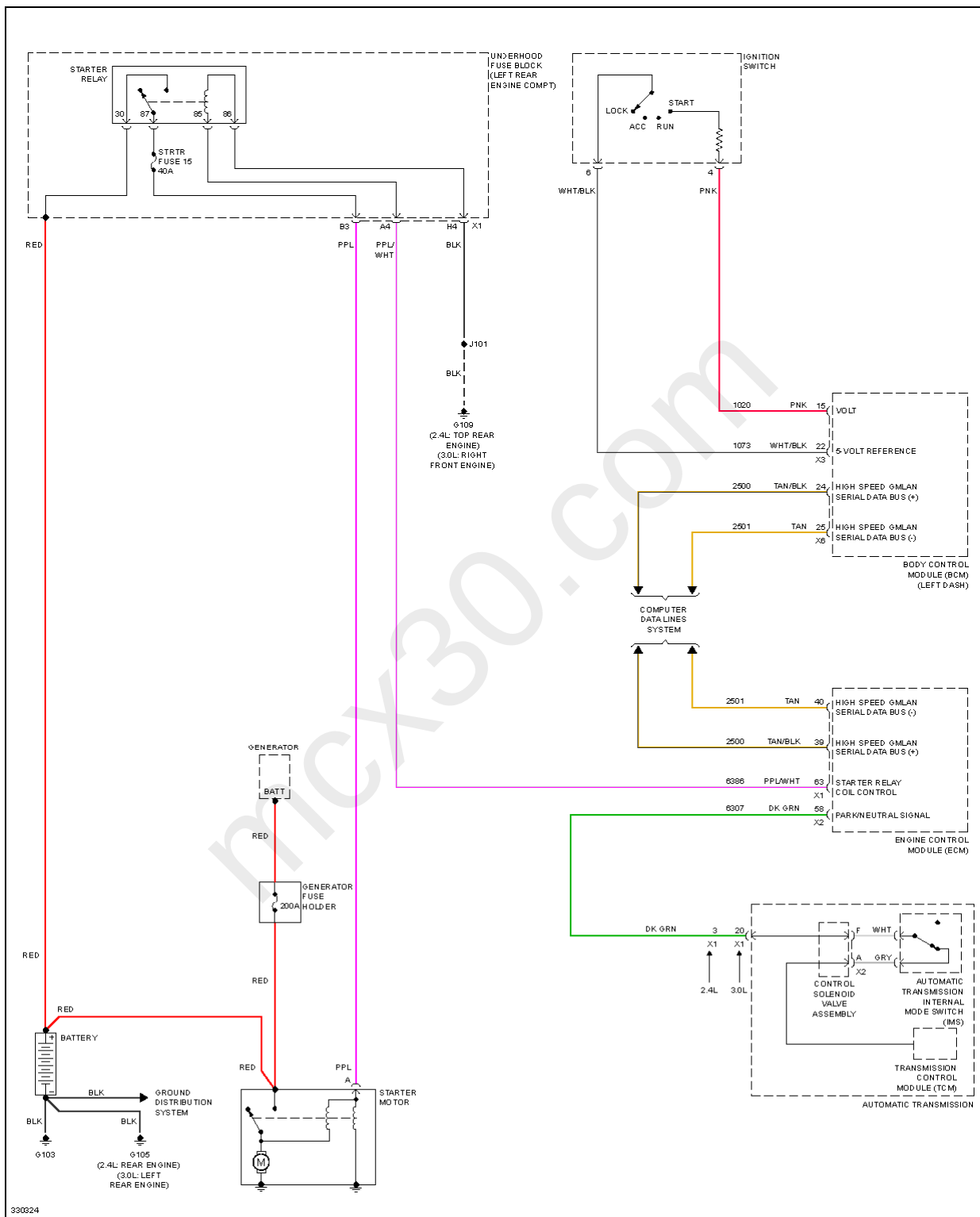
Fig. 72: Starting Circuit
