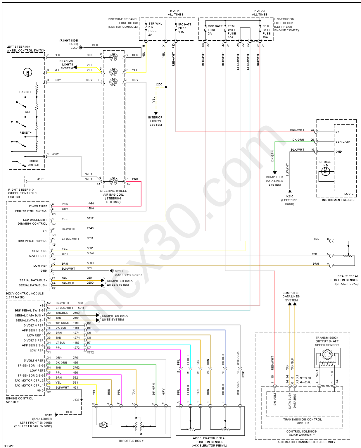
Fig. 16: Cruise Control Circuit
