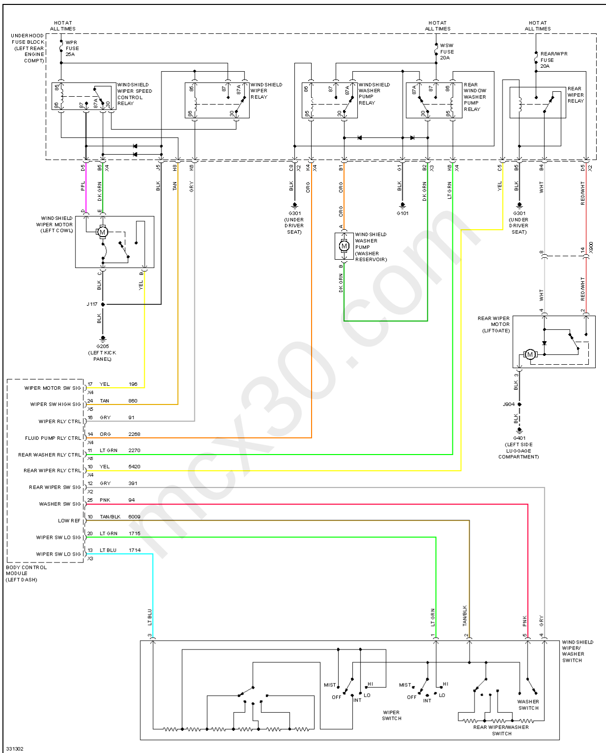
Fig. 82: Wiper/Washer Circuit
