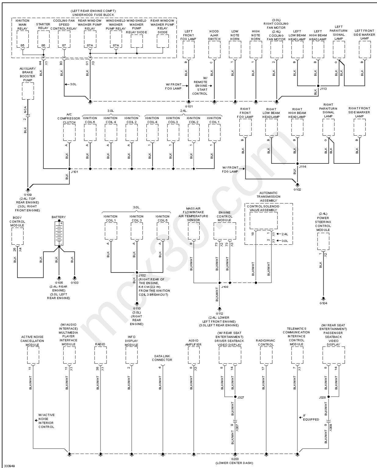
Fig. 32: Ground Distribution Circuit (1 of 4)
